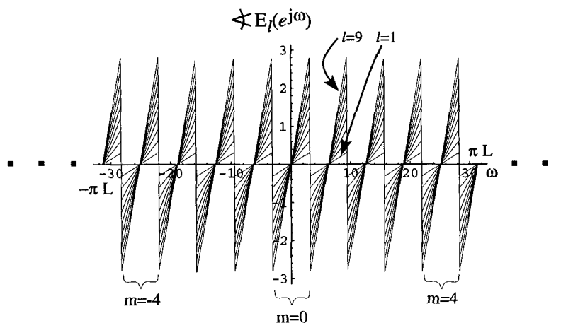
Fig. 42. Phase response of ideal polyphase filters E_l(e^{j\omega}) ; L = 10 .
