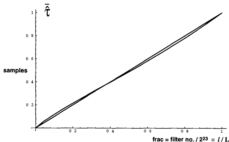
Fig. 31. Average delay of each all-pass interpolation polyphase filter.
