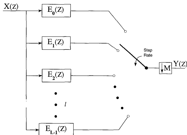
Fig. 41. Commutator model of classical polyphase interpolation showing numerous polyphase filters.
