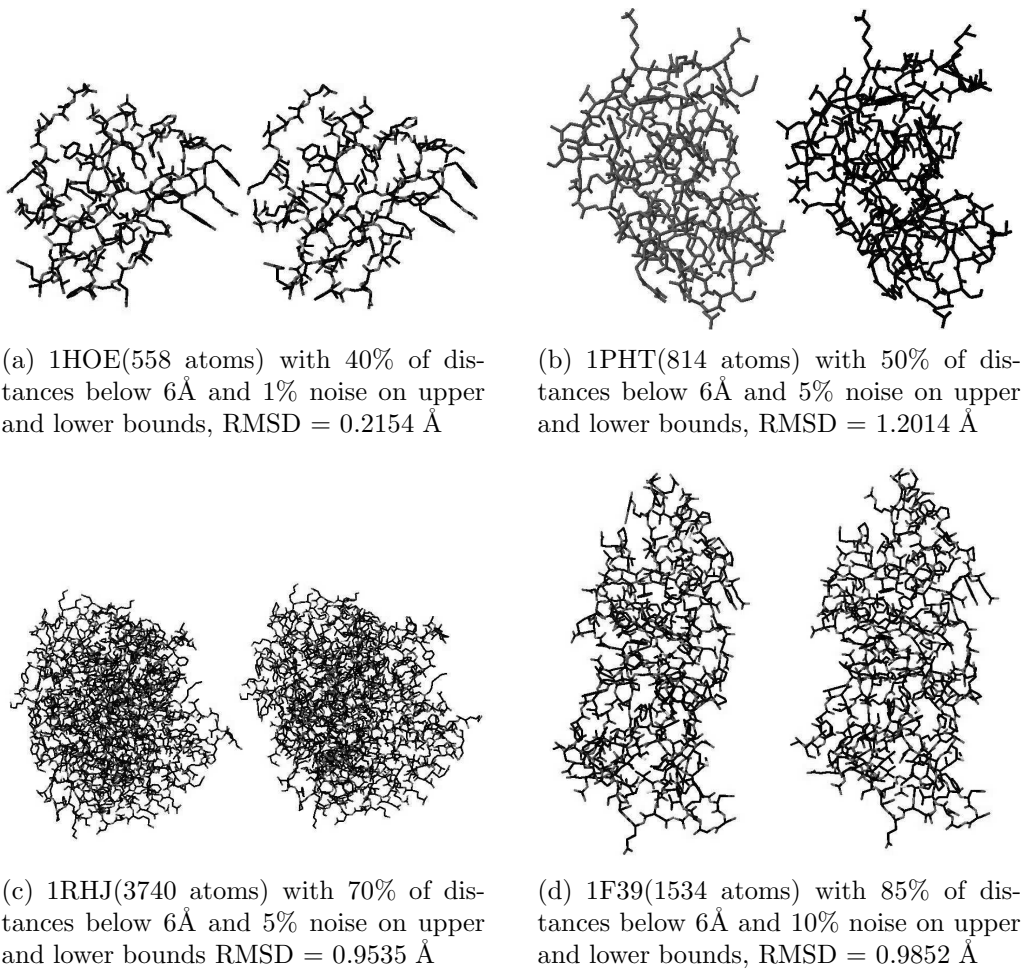
Figure 5: Comparison between the original (left) and reconstructed (right) configurations for various protein molecules using Swiss PDB viewer
