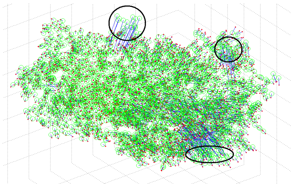
Figure 4: 1BPM(3672 atoms) with 50% of distances below 6Å and 5% noise on upper and lower bounds, RMSD = 2.4360 Å
