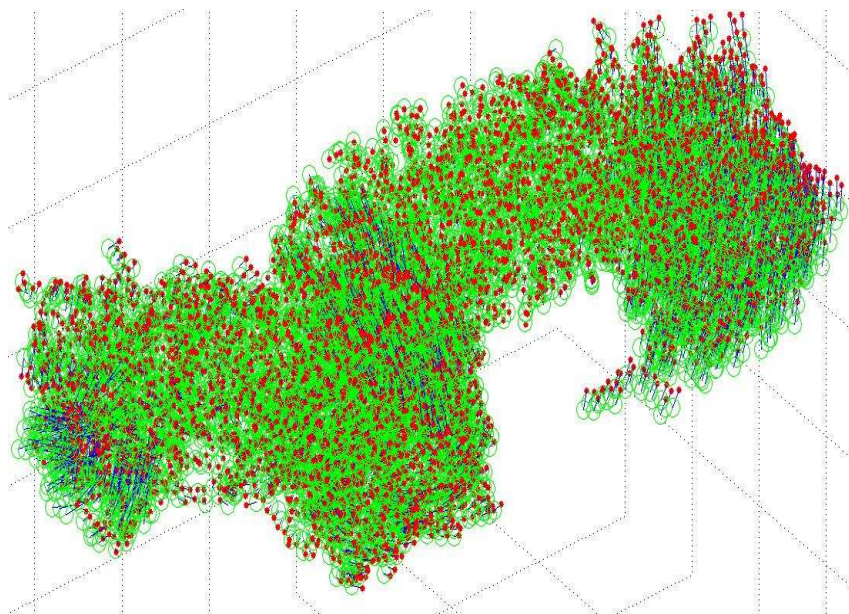
Figure 3: 1I7W(8629 atoms) with 100% of distances below 6Å and 10% noise on upper and lower bounds, RMSD = 1.3842 Å
